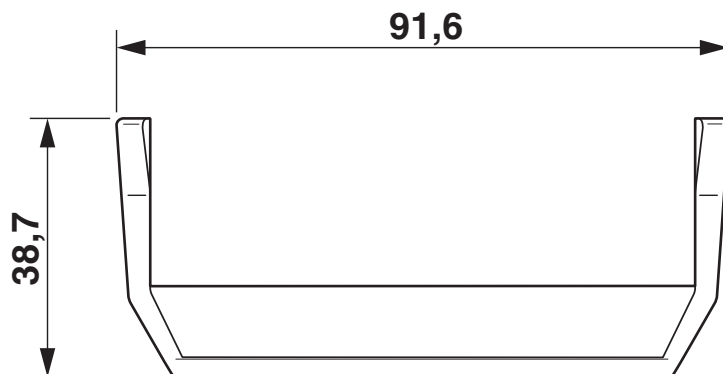
Dimensional drawing
